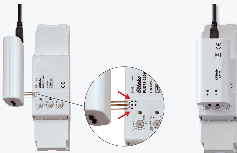
Plugging the data transformer DAT71 to a Series 71 actuator.
